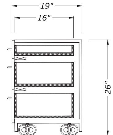
SECTION VIEW
