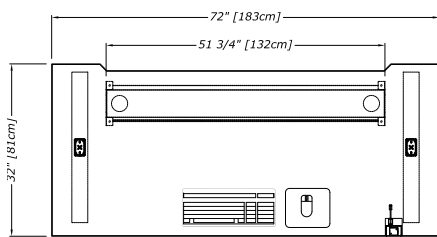
PLAN VIEW
